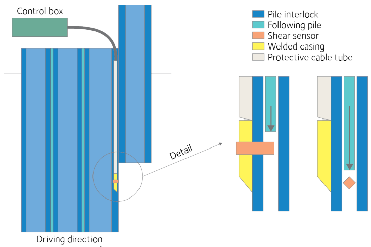
Schematic view of operating principle
