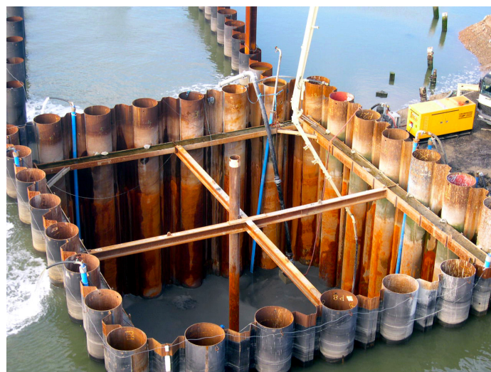
Watertight tubular combined wall Demey – Oostende (Belgium)
