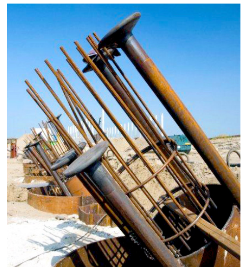
Example of a steel tube as anchoring element
