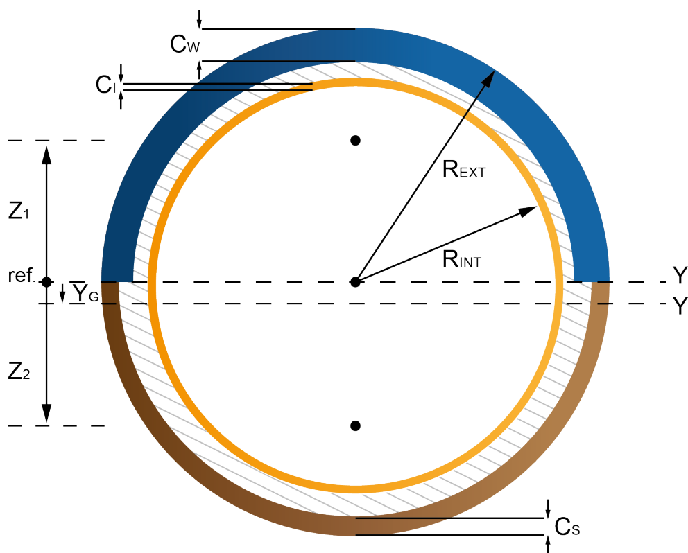
Figure: Tube surface with reduced area profile
