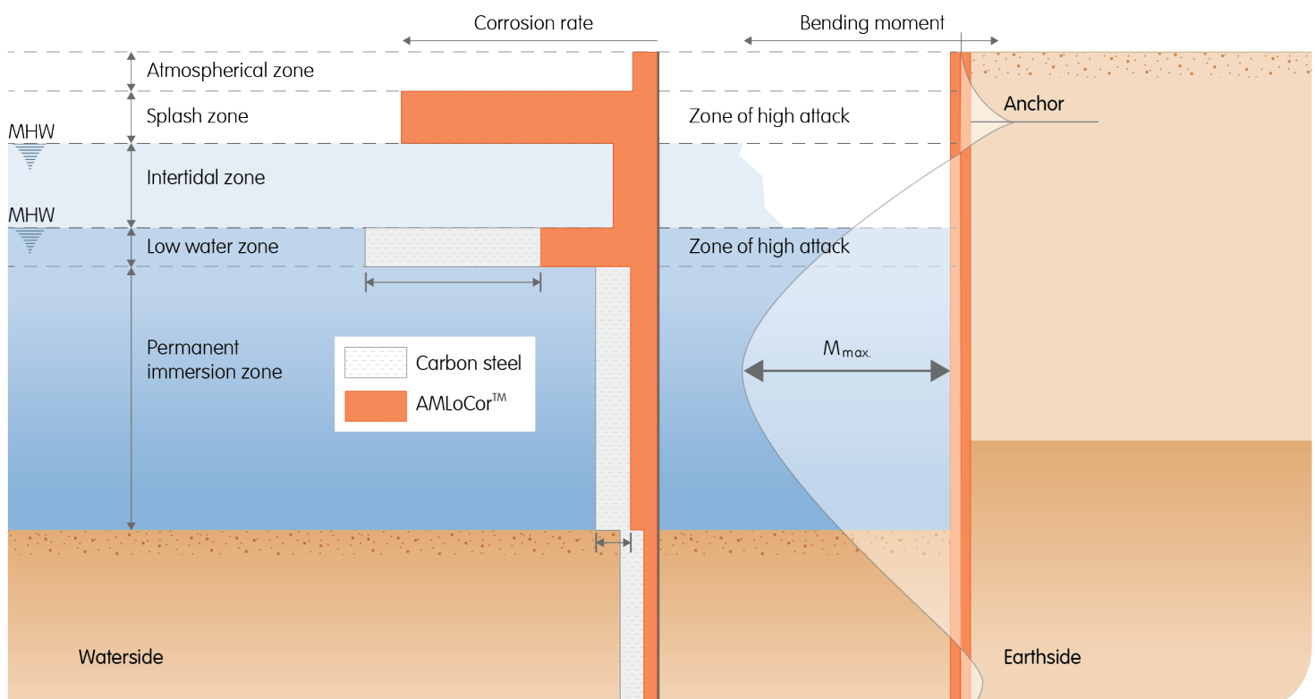
Typical loss of steel in a marine environment of carbon steel and AMLoCor™
