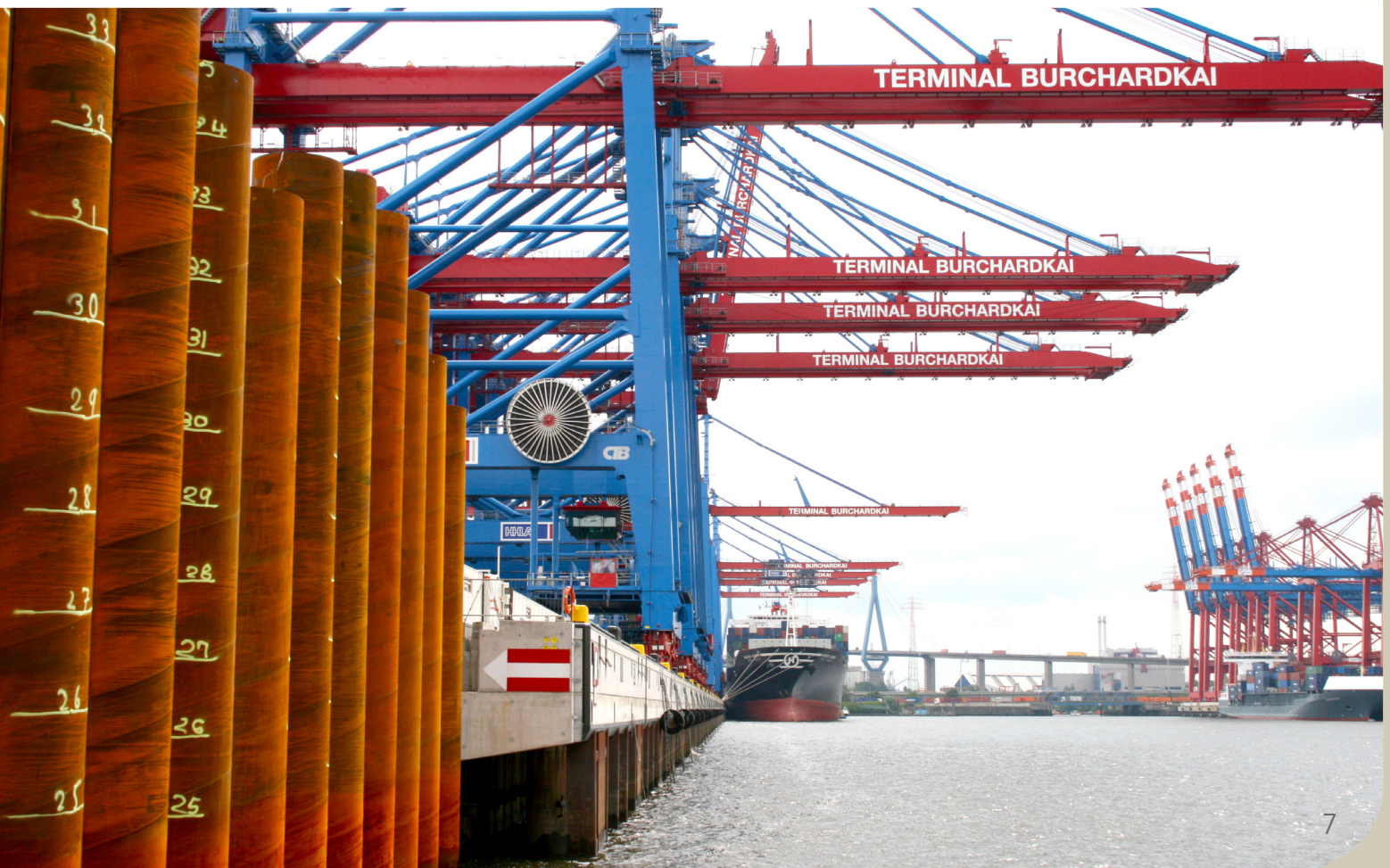
Keeping quay in operation during extension (Burchardkai, Germany)
