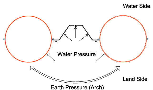
Arch effect of tubular combined wall
