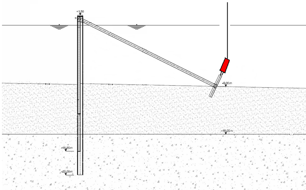
Vibro-driving of the anchor
