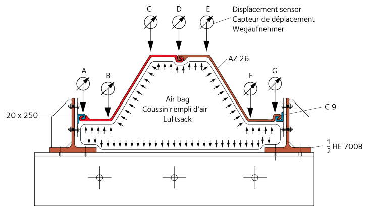
Resistance of sheet piles against high water pressures
