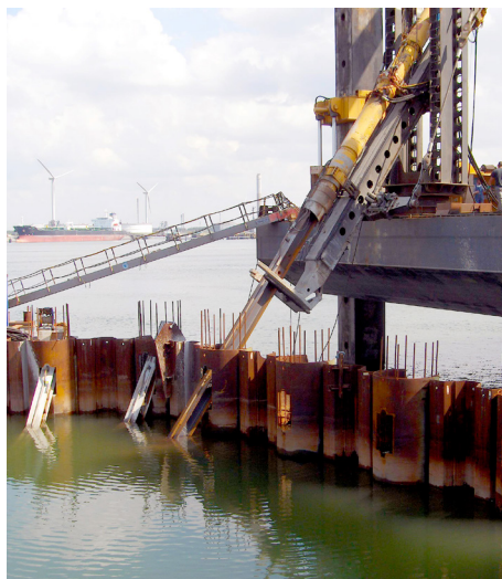
Installation of MV piles
