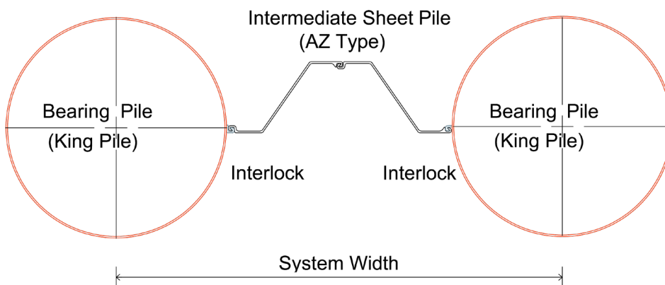
Tubular combined wall system with the different elements
