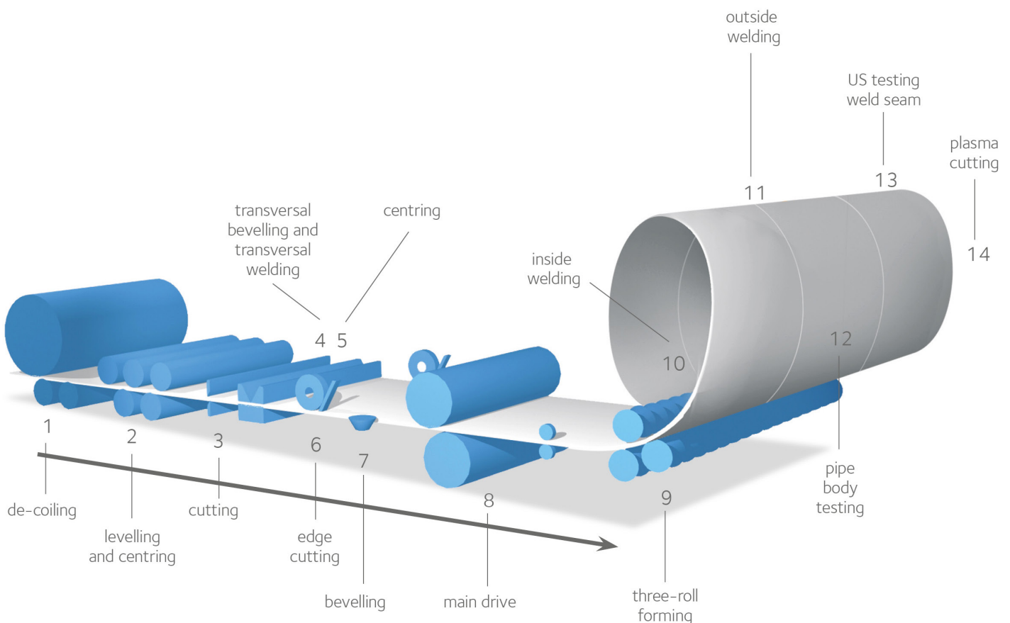
Production process of spirally welded pipes
